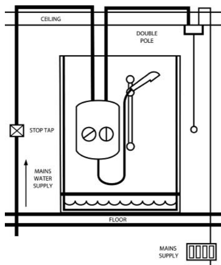
Typical Electric Shower Installation
