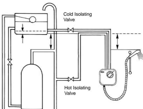
Typical Power Shower Installation
