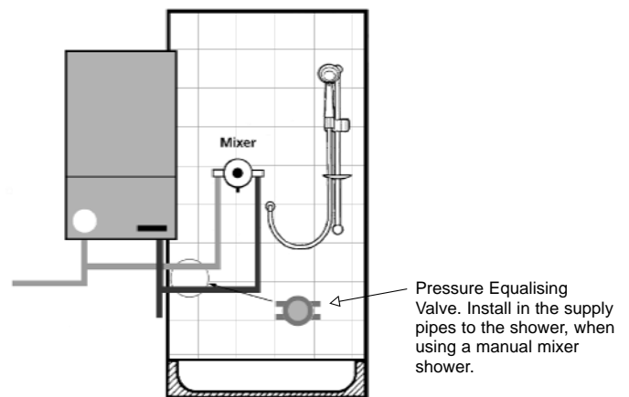
Typical Mains Pressure Shower Installation
