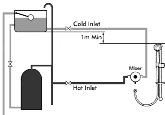
Typical Gravity Shower Installation
